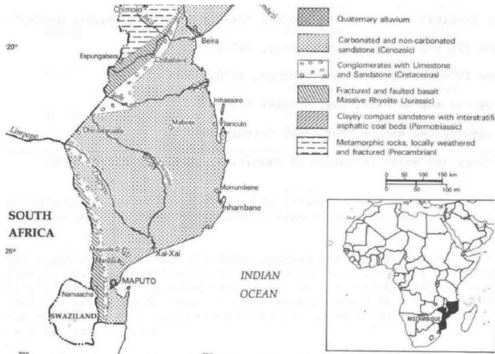
Figure 4. Main Geological and Lithological Units- Mozambique (Naturale resources. Water Series No. 19, 1989)
